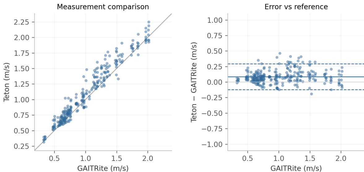
Figure 5: Walking speed pooled across recorded views. Each point is one paired camera-walk observation. Left: measurement comparison with identity line. Right: error versus reference, with mean bias (solid) and descriptive 95% limits of agreement (dashed). Reference and error axes use equal numerical spans.
