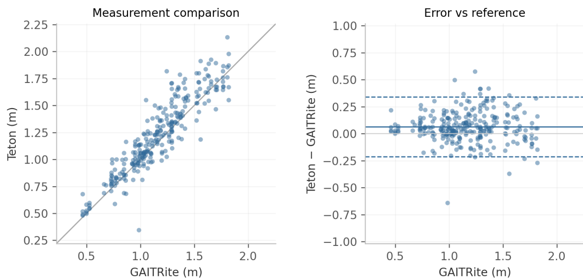
Figure 7: Stride length pooled across recorded views. Each point is one paired camera-walk observation. Left: measurement comparison with identity line. Right: error versus reference, with mean bias (solid) and descriptive 95% limits of agreement (dashed). Reference and error axes use equal numerical spans.
