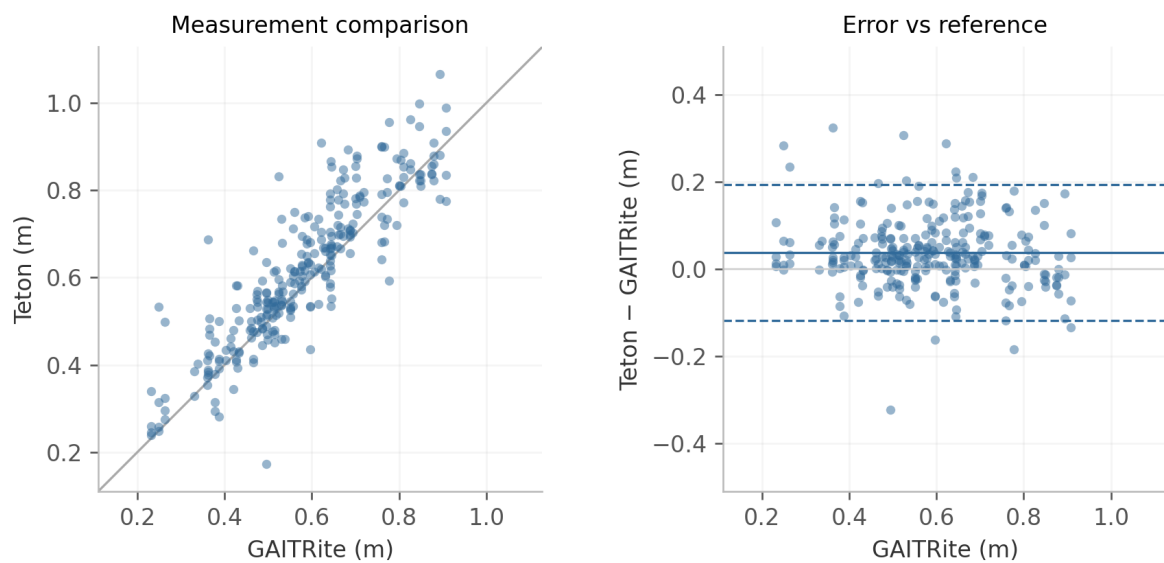
Figure 9: Step length pooled across recorded views. Each point is one paired camera-walk observation. Left: measurement comparison with identity line. Right: error versus reference, with mean bias (solid) and descriptive 95% limits of agreement (dashed). Reference and error axes use equal numerical spans.
