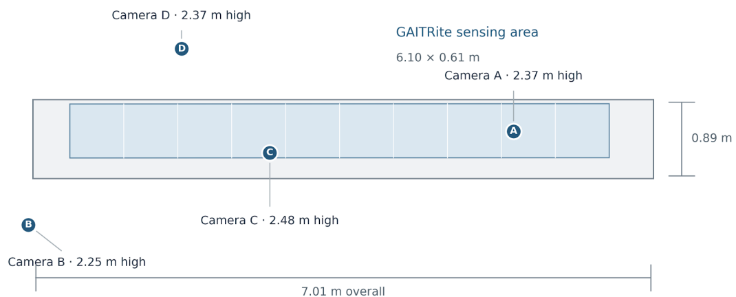
Figure 4: Camera and walkway layout, viewed from above. Camera markers show floor-projected positions from the shared calibration; labels give height above the floor. The blue region is the active sensing area. Horizontal distances are drawn to scale; camera symbols are schematic.
