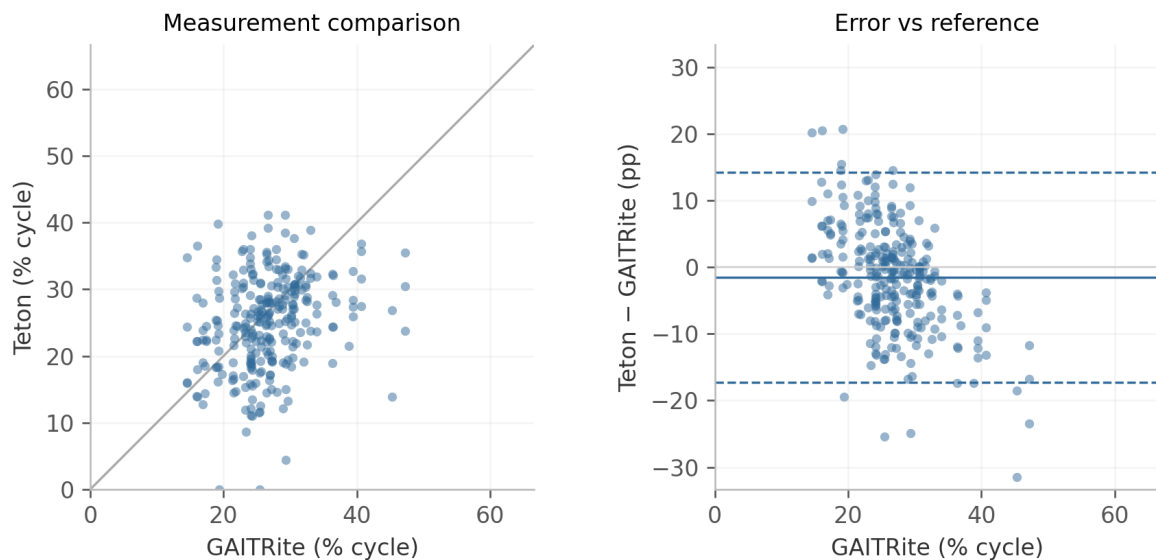
Figure 11: Double support time pooled across recorded views. Each point is one paired camera-walk observation. Left: measurement comparison with identity line. Right: error versus reference, with mean bias (solid) and descriptive 95% limits of agreement (dashed). Reference and error axes use equal numerical spans.
