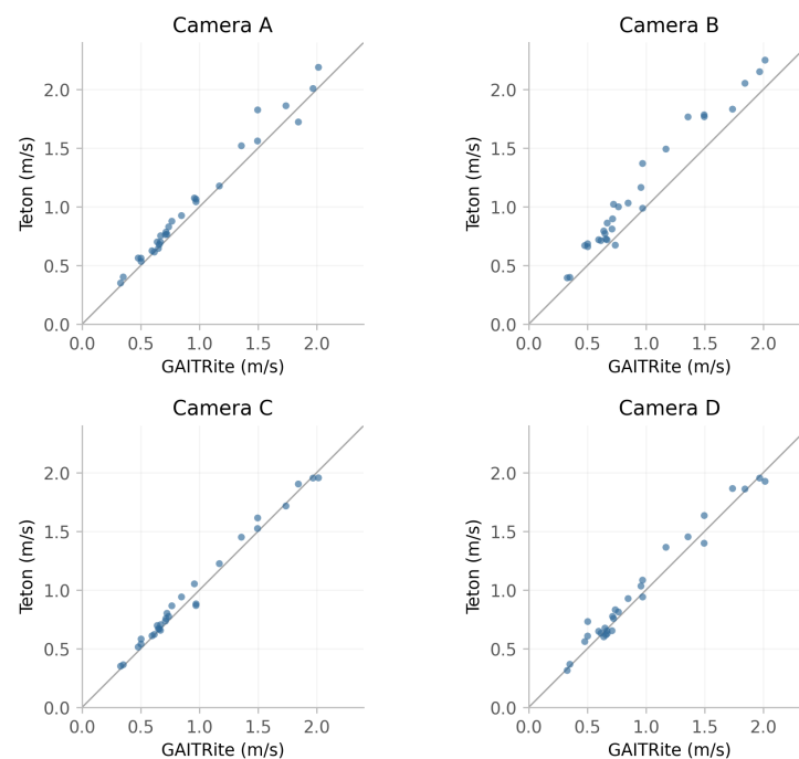
Figure A1: Walking-speed comparison for the same 29 walks in each camera view. Each point pairs a camera measurement with its GAITRite walk summary; the line indicates equality. All panels use identical axes.
