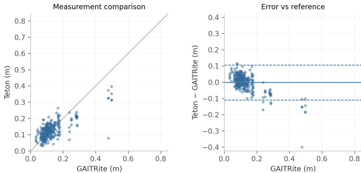
Figure 10: Step width pooled across recorded views. Each point is one paired camera-walk observation. Left: measurement comparison with identity line. Right: error versus reference, with mean bias (solid) and descriptive 95% limits of agreement (dashed). Reference and error axes use equal numerical spans.
