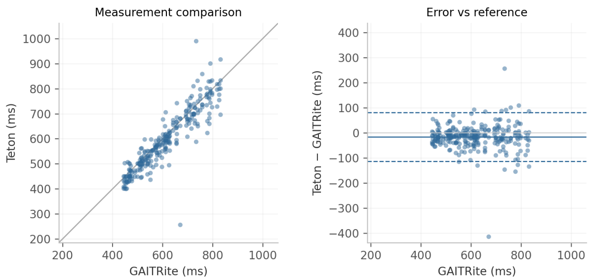
Figure 8: Step time pooled across recorded views. Each point is one paired camera-walk observation. Left: measurement comparison with identity line. Right: error versus reference, with mean bias (solid) and descriptive 95% limits of agreement (dashed). Reference and error axes use equal numerical spans.
