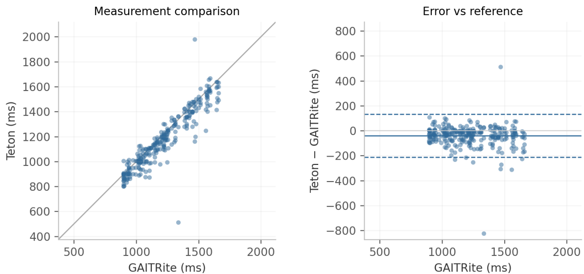
Figure 6: Stride time pooled across recorded views. Each point is one paired camera-walk observation. Left: measurement comparison with identity line. Right: error versus reference, with mean bias (solid) and descriptive 95% limits of agreement (dashed). Reference and error axes use equal numerical spans.
